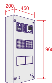
Large (2-4-6-8 loop) (12-38Ahr Batteries)
